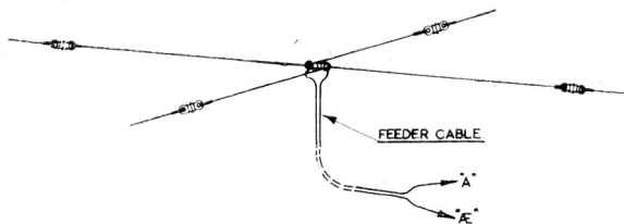
Fig. 3. Double dipole aerial, giving wider frequency coverage than a single dipole.
