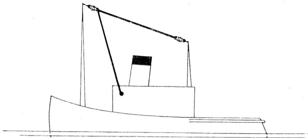
Fig. 10. A suitable aerial for use in a tug or similar vessel.
