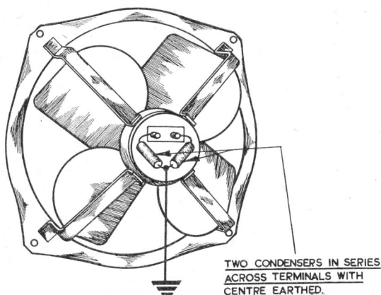
Fig. 15. An improved way of suppressing interference—two condensers in series with the centre earthed.
